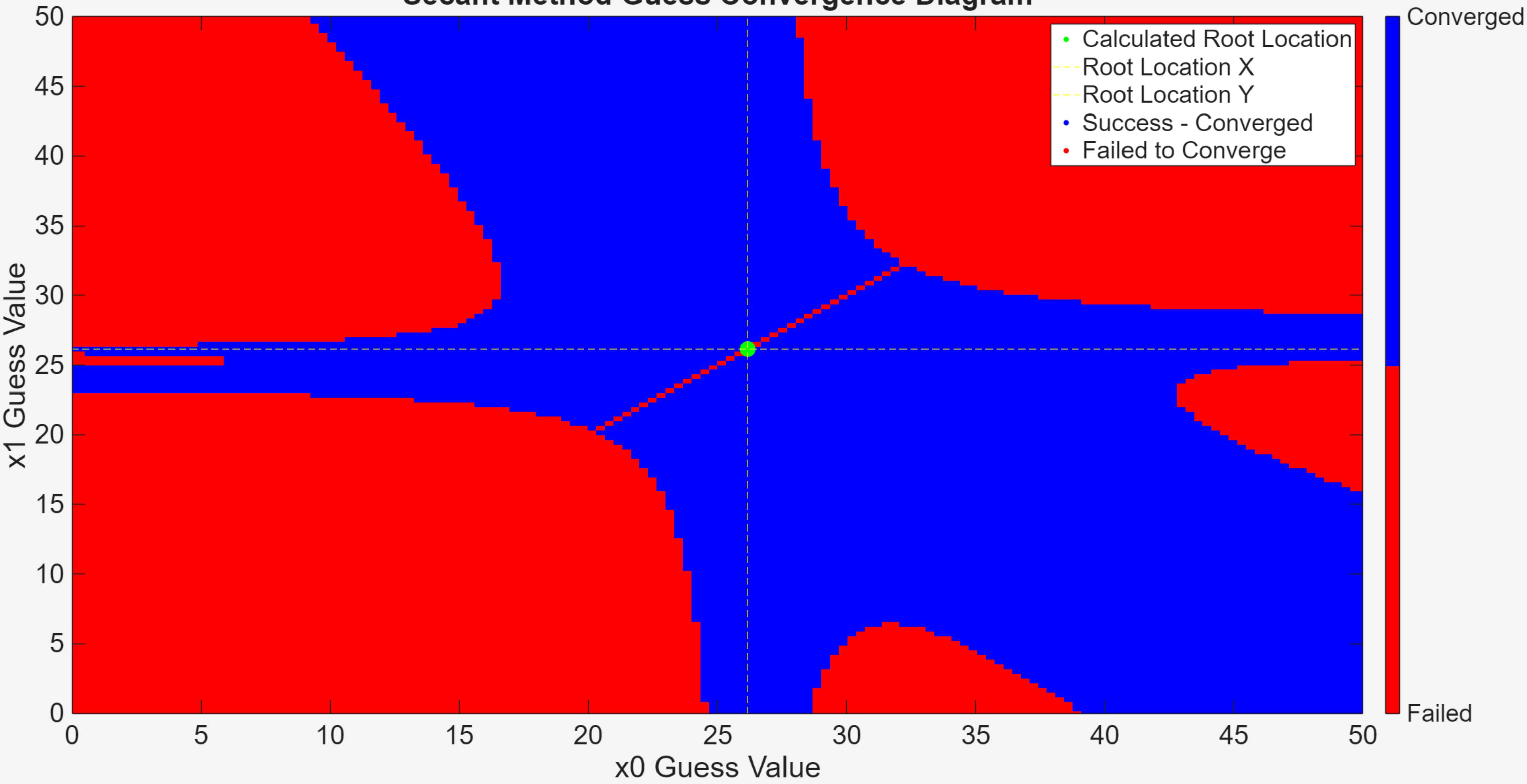
Secant Method Guess Convergence Diagram
